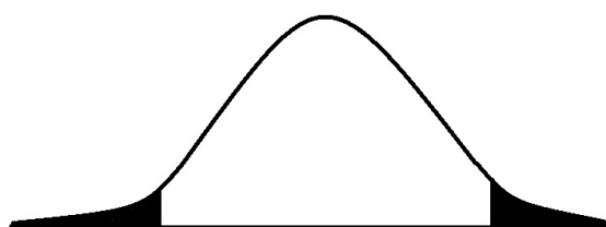
Figure 4.2 Two Tailed Test
