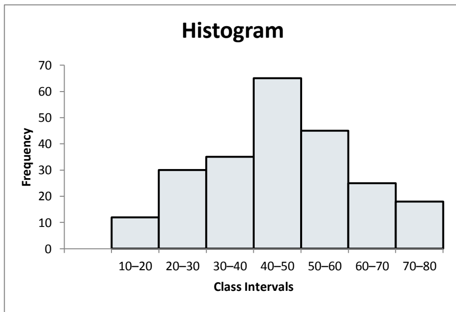
Figure 8: Histogram
