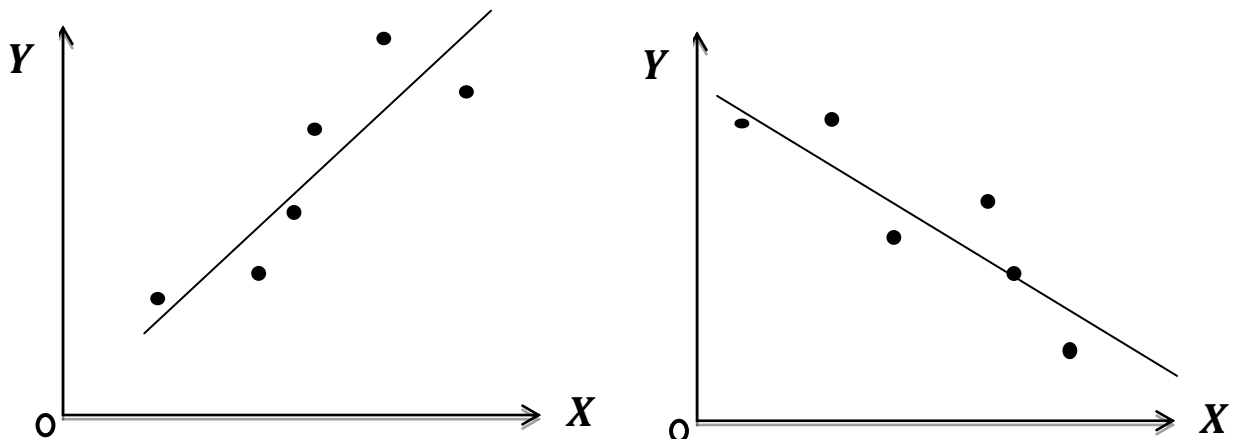
Figure 3.3 (a): High Degree of Positive Correlation Figure 3.3(b): High Degree of Negative Correlation
